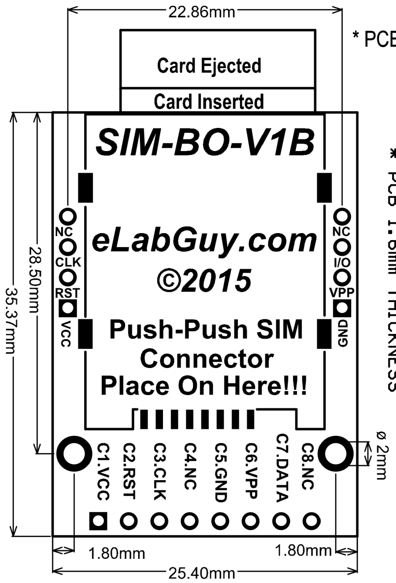
SIM-BO-V1B PCB outline Drawing
